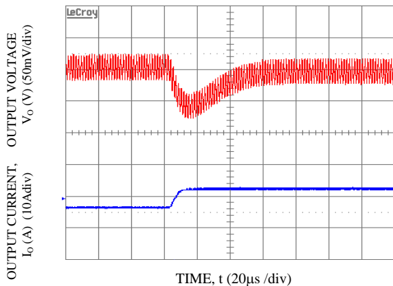
Figure 35. Transient Response to Dynamic Load Change from 50% to 100% at 12Vin, Cout-1x 47 µF + 1x 330 µF, CTune-2700 pF & RTune-330 ohms. Vo = 3.3 V
