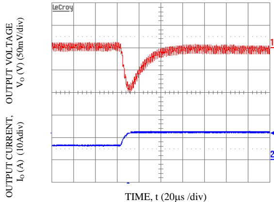
Figure 36. Transient Response to Dynamic Load Change from 50% to 100% at 12Vin, Cout-5x 47 µF, CTune-1500 pF & RTune-330 ohms. Vo = 5.0 V
