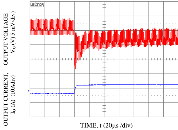
Figure 31. Transient Response to Dynamic Load Change from 50% to 100% at 12Vin, Cout-3x 47 µF + 6x 330 µF, CTune-47 nF, RTune-180 ohms. Vo = 0.6 V
