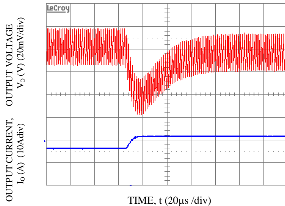
Figure 34. Transient Response to Dynamic Load Change from 50% to 100% at 12Vin, Cout-1x 47µF + 1x 330 µF, CTune-3300pF & RTune-270 ohms. Vo = 2.5 V
