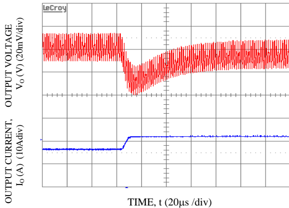
Figure 33. Transient Response to Dynamic Load Change from 50% to 100% at 12Vin, Cout-1x47µF+2x330µF, CTune-5600 pF & RTune-270 ohms. Vo = 1.8 V
