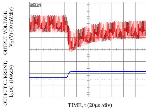
Figure 32. Transient Response to Dynamic Load Change from 50% to 100% at 12Vin, Cout-1x 47 µF + 3x 330 µF, CTune-10 nF & RTune-220 ohms. Vo = 1.2 V
