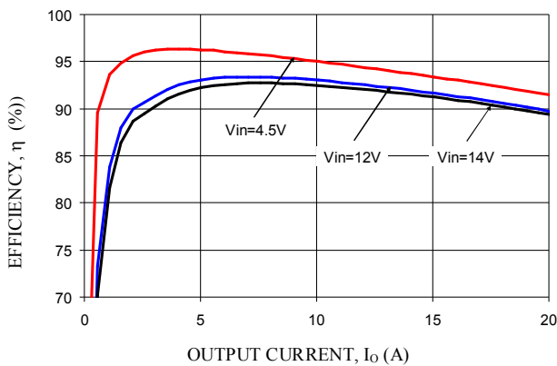
V_o = 3.3V
