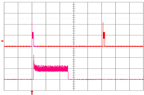
Fig. 18: Load current (top trace, 5 A/div., 20 ms/div.) into a 10 \text{ m}\Omega short circuit during restart, at V_{in} = 24 \text{ V} . Bottom trace (5 A/div., 1 ms/div.) is an expansion of the on-time portion of the top trace.
