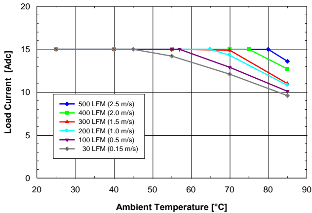
Fig. 3.3V.1: Available load current vs. ambient air temperature and airflow rates for SQ24T15033 converter with B height pins mounted vertically with V_{in} = 24V , air flowing vertically from pin 3 to pin 1 and maximum FET temperature \leq 120^{\circ}C .
