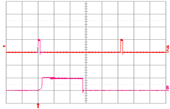
Fig. 3.3V.18: Load current (top trace, 20 A/div., 20 ms/div.) into a 10 \text{m}\Omega short circuit during restart, at V_{in} = 24 \text{ V} . Bottom trace (20 A/div., 1 ms/div.) is an expansion of the on-time portion of the top trace.
