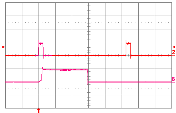
Fig. 1.8V.18: Load current (top trace, 20 A/div., 20 ms/div.) into a 10 \text{m}\Omega short circuit during restart, at V_{in} = 24 \text{ V} . Bottom trace (20 A/div., 2 ms/div.) is an expansion of the on-time portion of the top trace.
