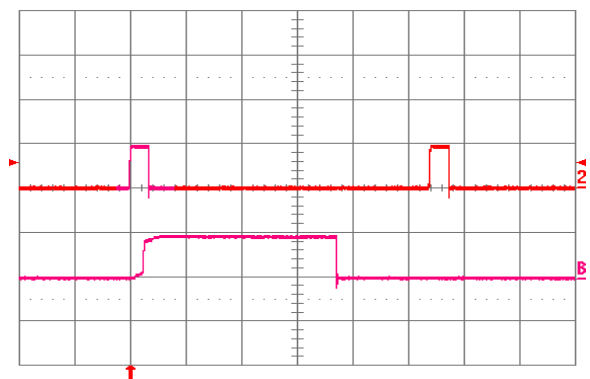
Fig. 1.0V.18: Load current (top trace, 20 A/div., 20 ms/div.) into a 10 m \Omega short circuit during restart, at V_{in} = 24 \text{ V} . Bottom trace (20 A/div., 2 ns/div.) is an expansion of the on-time portion of the top trace.
