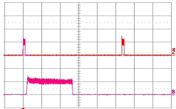
Fig. 12V.18: Load current (top trace, 5 A/div., 20 ms/div.) into a 10 \text{ m}\Omega short circuit during restart, at V_{in} = 24 \text{ V} . Bottom trace (5 A/div., 1 ms/div.) is an expansion of the on-time portion of the top trace.
