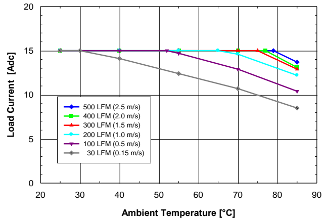
Fig. 3.3V.2: Available load current vs. ambient air temperature and airflow rates for SQ24T15033 converter with B height pins mounted horizontally with V_{in} = 24V , air flowing horizontally from pin 3 to pin 1 and maximum FET temperature \leq 120^{\circ}C .
