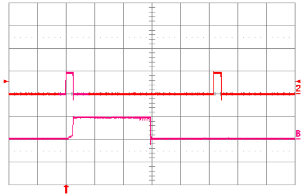
Fig. 1.2V.18: Load current (top trace, 20 A/div., 20 ms/div.) into a 10 m \Omega short circuit during restart, at V_{in} = 24 \text{ V} . Bottom trace (20 A/div., 2 ms/div.) is an expansion of the on-time portion of the top trace.
