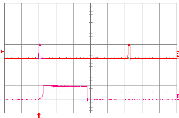
Fig. 3.3V.18: Load current (top trace, 20 A/div., 20 ms/div.) into a 10 \text{ m}\Omega short circuit during restart, at V_{in} = 24\text{V} . Bottom trace (20 A/div., 1 ms/div.) is an expansion of the on-time portion of the top trace.
