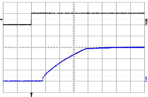
Fig. 6.0V.10: Turn-on transient at full rated load current (resistive) plus 10,000 \mu\text{F} at V_{in} = 24\text{V} , triggered via ON/OFF pin. Top trace: ON/OFF signal (5 V/div.). Bottom trace: output voltage (2 V/div.). Time scale: 2 ms/div.
