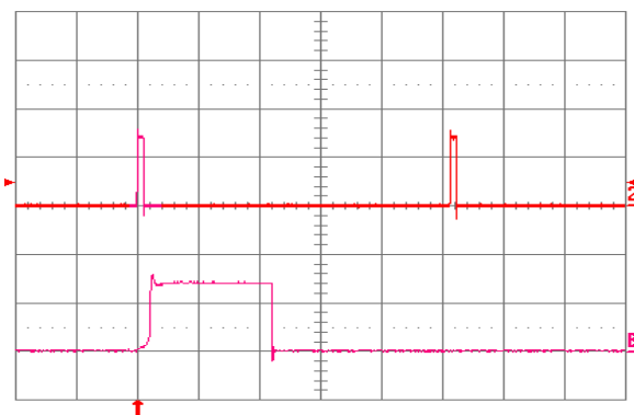
Fig. 5.0V.18: Load current (top trace, 10 A/div., 20 ms/div.) into a 10 \text{ m}\Omega short circuit during restart, at V_{in} = 24\text{V} . Bottom trace (10 A/div., 1 ms/div.) is an expansion of the on-time portion of the top trace.
