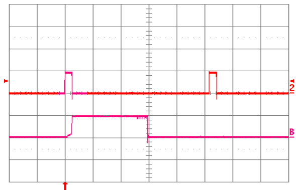
Fig. 1.2V.18: Load current (top trace, 20 \text{ A}/\text{div} ., 20 \text{ ms}/\text{div} .) into a 10 \text{ m}\Omega short circuit during restart, at V_{in} = 24\text{V} . Bottom trace ( 20 \text{ A}/\text{div} ., 2 \text{ ms}/\text{div} .) is an expansion of the on-time portion of the top trace.
