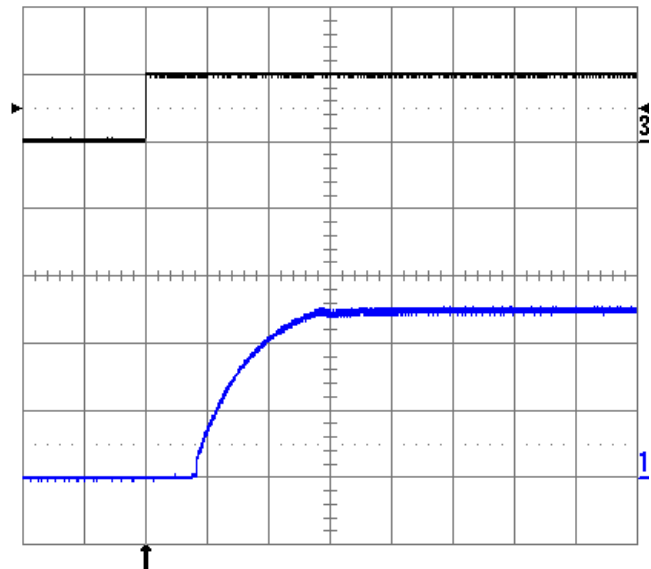
Fig. 2.5V.10: Turn-on transient at full rated load current (resistive) plus 10,000 \mu\text{F} at V_{in} = 48\text{ V} , triggered via ON/OFF pin. Top trace: ON/OFF signal (5 V/div.). Bottom trace: output voltage (1 V/div.). Time scale: 2 ms/div.
