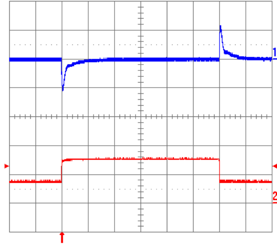
Fig. 1.2V.12: Output voltage response to load current step-change (3.75 A – 7.5 A – 3.75 A) at V_{in} = 48 V. Top trace: output voltage (100 mV/div.). Bottom trace: load current (5 A/div.). Current slew rate: 5 A/ \mu s. C_o = 450 \mu F tantalum + 1 \mu F ceramic. Time scale: 0.2 ms/div.
