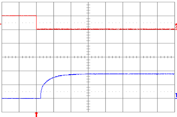
Fig. 1.8V.7: Turn-on transient at full rated load current (resistive) with no output capacitor at V_{in} = 48\text{ V} , triggered via ON/OFF pin. Top trace: ON/OFF signal (5 V/div.). Bottom trace: Output voltage (1 V/div.). Time scale: 2 ms/div.
