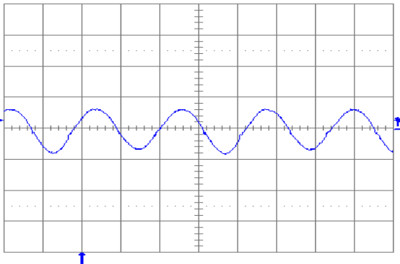
Fig. 2.5V.11: Output voltage ripple (20 mV/div.) at full rated load current into a resistive load with C_o = 10 \mu F tantalum + 1 \mu F ceramic and V_{in} = 48 V. Time scale: 1 \mu s/div.
