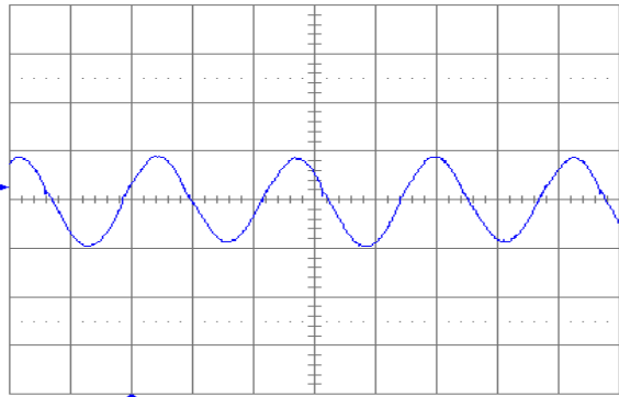
Fig. 3.3V.11: Output voltage ripple (20 mV/div.) at full rated load current into a resistive load with C_o = 10 \mu\text{F} tantalum + 1 \mu\text{F} ceramic and V_{in} = 48 \text{ V} . Time scale: 1 \mu\text{s}/\text{div.} .
