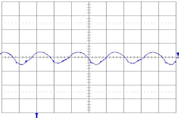
Fig. 1.5V.11: Output voltage ripple (20 mV/div.) at full rated load current into a resistive load with C_o = 10 \mu F tantalum + 1 \mu F ceramic and V_{in} = 48 V. Time scale: 1 \mu s/div.
