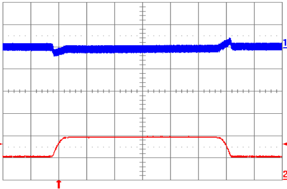
Fig. 2.5V.9: Output voltage response to load current step-change (10 A – 20 A – 10 A) at V_{in} = 48 V. Top trace: output voltage (100 mV/div.). Bottom trace: load current (10 A/div.). Current slew rate: 0.1 A/ \mu s. C_o = 1 \mu F ceramic. Time scale: 0.2 ms/div.
