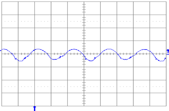
Fig. 1.2V.11: Output voltage ripple (20 mV/div.) at full rated load current into a resistive load with C_o = 10 \mu F tantalum + 1 \mu F ceramic and V_{in} = 48 V. Time scale: 1 \mu s/div.
