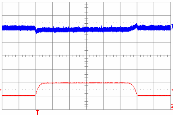
Fig. 3.3V.9: Output voltage response to load current step-change (10 A – 20 A – 10 A) at V_{in} = 48\text{ V} . Top trace: output voltage (100 mV/div.). Bottom trace: load current (10 A/div.). Current slew rate: 0.1 A/ \mu\text{s} . C_o = 1\ \mu\text{F} ceramic. Time scale: 0.2 ms/div.
