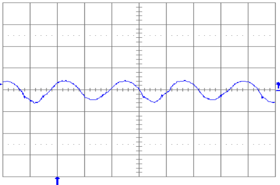
Fig. 1.8V.11: Output voltage ripple (20 mV/div.) at full rated load current into a resistive load with C_o = 10 \mu F tantalum + 1 \mu F ceramic and V_{in} = 48 V. Time scale: 1 \mu s/div.
