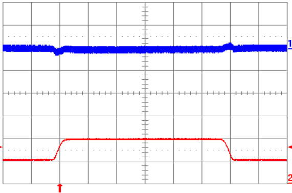
Fig. 1.5V.9: Output voltage response to load current step-change (10 A – 20 A – 10 A) at V_{in} = 48 V. Top trace: output voltage (100 mV/div.). Bottom trace: load current (10 A/div.). Current slew rate: 0.1 A/ \mu s. C_o = 1 \mu F ceramic. Time scale: 0.2 ms/div.
