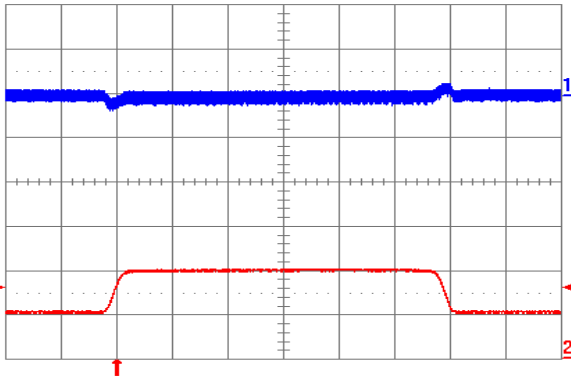
Fig. 1.2V.9: Output voltage response to load current step-change (10 A – 20 A – 10 A) at V_{in} = 48 V. Top trace: output voltage (100 mV/div.). Bottom trace: load current (10 A/div.). Current slew rate: 0.1 A/ \mu s. C_o = 1 \mu F ceramic. Time scale: 0.2 ms/div.
