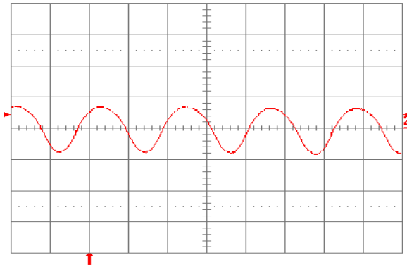
Fig. 1.8V.13: Input reflected-ripple current, i_c (100 mA/div.), measured at input terminals at full rated load current and V_{in} = 48 V. Refer to Fig. 1.8V.12 for test setup. Time scale: 1 \mu s/div.
