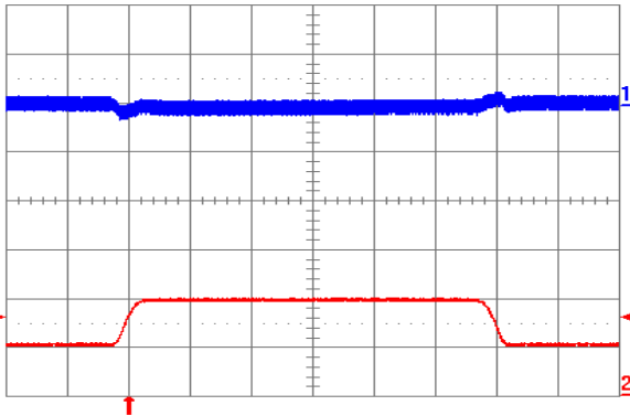
Fig. 1.8V.9: Output voltage response to load current step-change (10 A – 20 A – 10 A) at V_{in} = 48 V. Top trace: output voltage (100 mV/div.). Bottom trace: load current (10 A/div.). Current slew rate: 0.1 A/ \mu s. C_o = 1 \mu F ceramic. Time scale: 0.2 ms/div.
