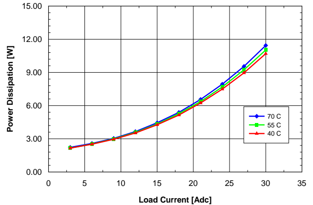
Fig. 3.3V.6: Power dissipation vs. load current and ambient temperature with V_{in} = 48\text{ V} and air flowing from pin 3 to pin 1 at a rate of 200 LFM (1.0 m/s).
