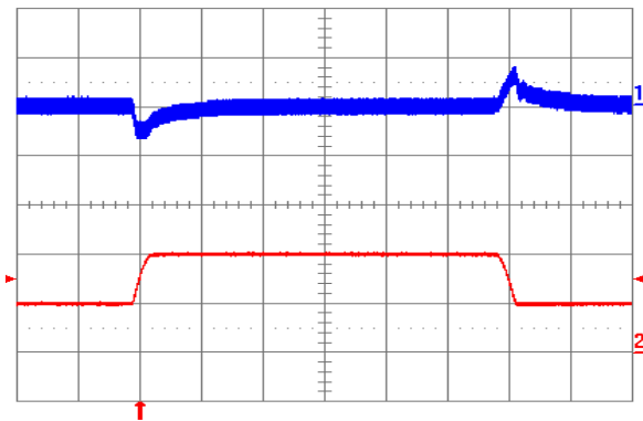
Fig. 2.0V.5: Output voltage response to load current step-change (5A – 10A – 5A) at V_{in} = 48\text{ V} . Top trace: output voltage (100 mV/div.). Bottom trace: load current (5A/div.). Current slew rate: 0.1 A/ \mu\text{s} . C_o = 1\ \mu\text{F} ceramic. Time scale: 0.2 ms/div.
