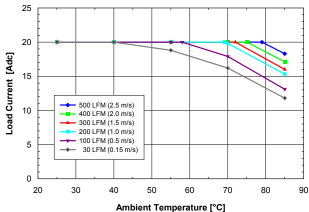
Fig. 1.5V.1: Available load current vs. ambient air temperature and airflow rates for SQM48T20015 converter with D height pins mounted vertically with air flowing from pin 3 to pin 1, MOSFET temperature \leq 120\text{ }^\circ\text{C} , V_{in} = 48\text{ V} .
