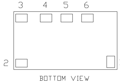
Figure 32. Pins
