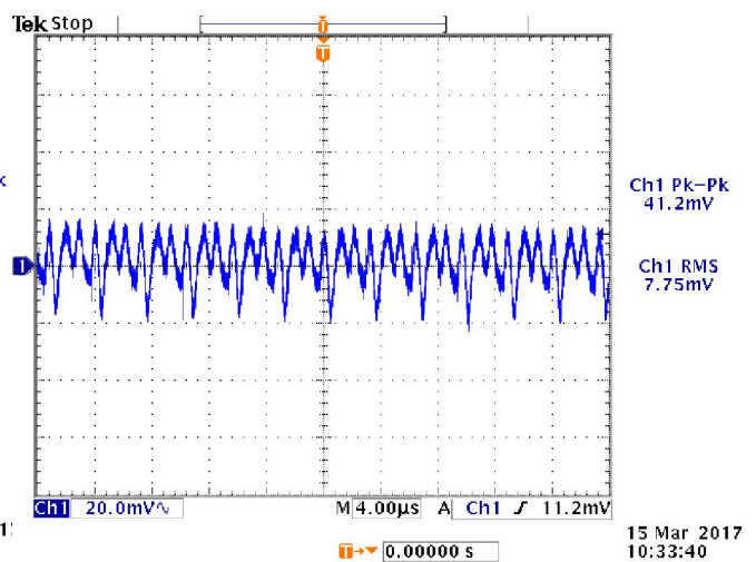
Ripple and noise at full load, V_{in}=24V
