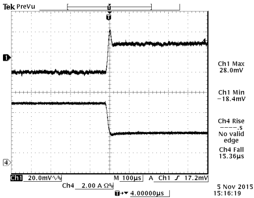
Figure 13. 100%-50% Load Transients at V_{in}=12\text{V} , V_{out}=3.3\text{V}@T_a=25^\circ\text{C}
