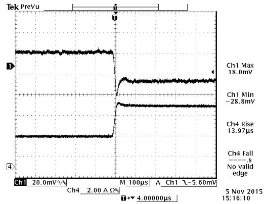
Figure 16. 50%-100% Load Transients at V_{in}=12V , V_{out}=5.5V@T_a=25^\circ C
