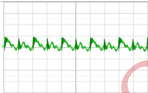
Figure 13. Output voltage ripple (20 mV/div.) at full rated load current into a resistive load with C_o = 10 μF tantalum + 1 μF ceramic and V_{in} = 48 V. Time scale: 2 μs/div.
