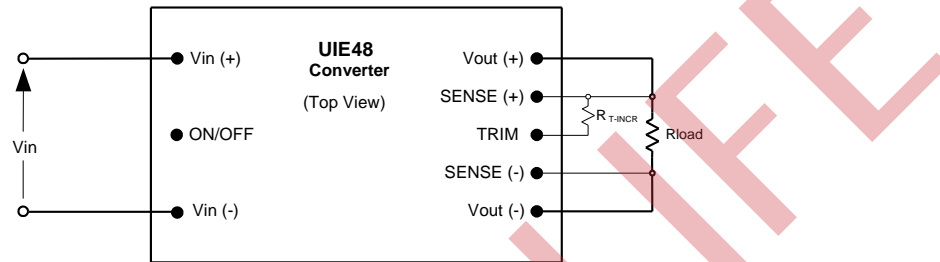
Fig. C: Configuration for increasing output voltage.
