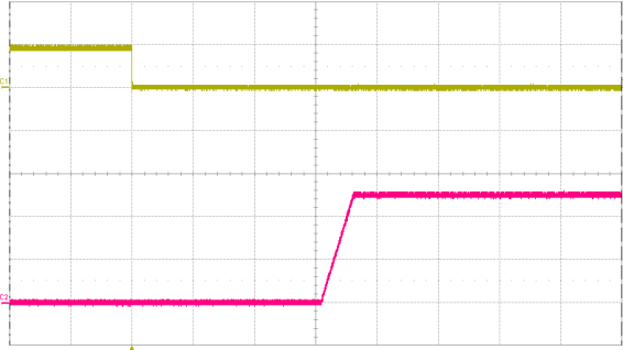
Fig. 9: Turn-on transient at full rated load current (resistive) with C_{out} 10\ \mu\text{F} tantalum + 1\ \mu\text{F} ceramic at V_{in} = 48\ \text{V} , triggered via ON/OFF pin. Top trace: ON/OFF signal (5 V/div.). Bottom trace: output voltage (2 V/div.). Time scale: 20 ms/div.
