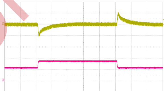
Fig. 12: Output voltage response to load current step change (12A – 18A – 12A) at V_{in} = 48\ \text{V} . Top trace: output voltage (200 mV/div.). Bottom trace: load current (10 A/div.). Current slew rate: 1\ \text{A}/\mu\text{s} . C_o = 1\ \mu\text{F} ceramic + 4,700\ \mu\text{F} + 10\ \mu\text{F} tantalum. Time scale: 200 \mu\text{s} /div.
