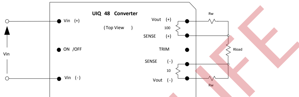
Fig. B: Remote sense circuit configuration.
