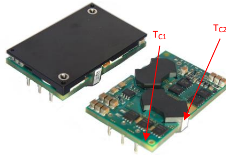
Fig. G: Locations of the thermocouples for thermal testing.
