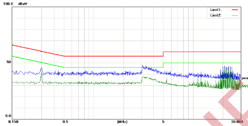
Fig. 19: Vin+ Peak Detector EMI waveform
