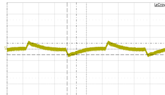
Fig. 12: Output voltage response to load current step-change ( 7 \text{ A} - 10.5 \text{ A} - 7 \text{ A} ) at V_{in} = 48 \text{ V} . Current slew rate: 0.1 \text{ A}/\mu\text{s} . C_o = 470 \mu\text{F} E-cap + 1 \mu\text{F} ceramic + 10 \mu\text{F} tantalum. Time scale: 500 \mu\text{s}/\text{div} .
