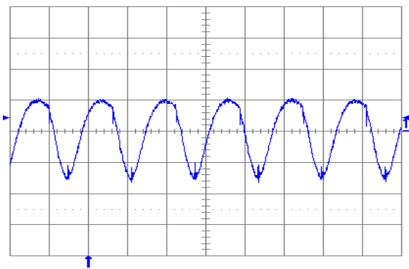
Fig. 3.3V.6: Output voltage ripple (20 mV/div.) at full rated load current into a resistive load with external capacitance 10\ \mu\text{F} ceramic + 1\ \mu\text{F} ceramic and V_{in} = 5\text{ V} for V_{out} = 3.3\text{ V} . Time scale: 2 μs/div.
