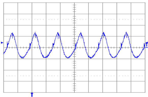
Fig. 1.0V.6: Output voltage ripple (20 mV/div.) at full rated load current into a resistive load with external capacitance 10 \mu\text{F} ceramic + 1 \mu\text{F} ceramic and V_{in} = 5 V for V_{out} = 1.0 V. Time scale: 2 \mu\text{s} /div.
