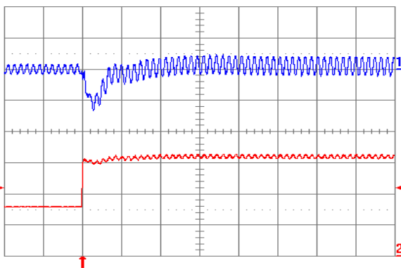
Fig. 2.0V.7: Output voltage response for V_{out} = 2.0\text{ V} to positive load current step change from 2.5 A to 5 A with slew rate of 5 A/ \mu\text{s} at V_{in} = 5\text{ V} . Top trace: output voltage (100 mV/div.); Bottom trace: load current (2 A/div.). C_o = 47\text{ }\mu\text{F} ceramic + 1 \mu\text{F} ceramic. Time scale: 20 \mu\text{s} /div.
