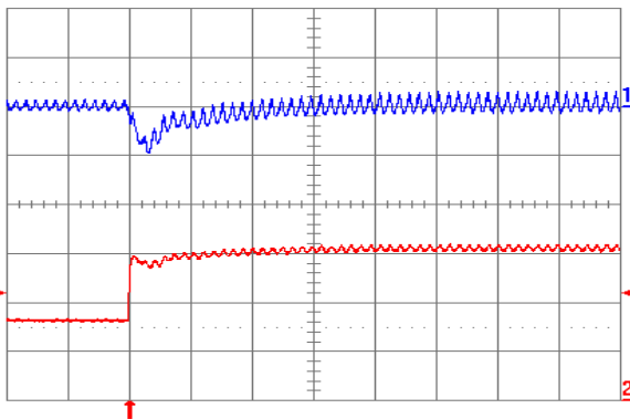
Fig. 0.7525V.7: Output voltage response for V_{out} = 0.7525 V to positive load current step change from 2.5 A to 5 A with slew rate of 5 A/ \mu\text{s} at V_{in} = 5 V. Top trace: output voltage (100 mV/div.); Bottom trace: load current (2 A/div.). C_o = 47 \mu\text{F} ceramic + 1 \mu\text{F} ceramic. Time scale: 20 \mu\text{s} /div.
