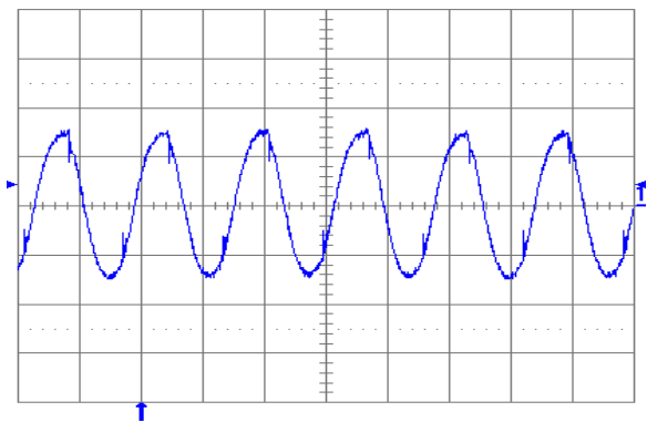
Fig. 2.0V.6: Output voltage ripple (20 mV/div.) at full rated load current into a resistive load with external capacitance 10 \mu\text{F} ceramic + 1 \mu\text{F} ceramic and V_{in} = 5\text{ V} for V_{out} = 2.0\text{ V} . Time scale: 2 \mu\text{s} /div.
