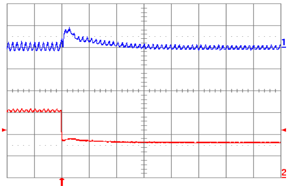
Fig. 0.7525V.8: Output voltage response for V_{out} = 0.7525 V to negative load current step change from 5 A to 2.5 A with slew rate of -5 A/ \mu\text{s} at V_{in} = 5 V. Top trace: output voltage (100 mV/div.); Bottom trace: load current (2 A/div.). C_o = 47 \mu\text{F} ceramic + 1 \mu\text{F} ceramic. Time scale: 20 \mu\text{s} /div.
