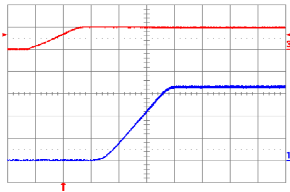
Fig. 3.3V.5: Turn-on transient for V_{out} = 3.3\text{ V} with application of V_{in} at full rated load current (resistive) and 47\ \mu\text{F} external capacitance at V_{in} = 5\text{ V} . Top trace: V_{in} (5 V/div.); Bottom trace: output voltage (1V/div.); Time scale: 2 ms/div.
