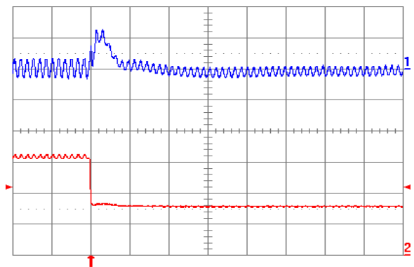
Fig. 2.0V.8: Output voltage response for V_{out} = 2.0\text{ V} to negative load current step change from 5 A to 2.5 A with slew rate of -5 A/ \mu\text{s} at V_{in} = 5\text{ V} . Top trace: output voltage (100 mV/div.); Bottom trace: load current (2 A/div.). C_o = 47\text{ }\mu\text{F} ceramic + 1 \mu\text{F} ceramic. Time scale: 20 \mu\text{s} /div.
