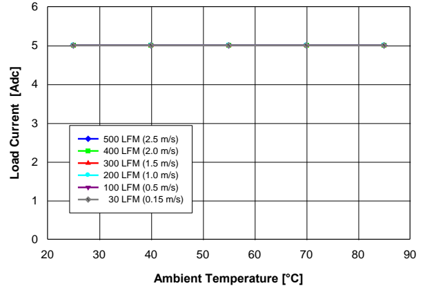
Fig. 1.2V.2: Available load current vs. ambient temperature and airflow rates for V_{out} = 1.2\text{V} converter mounted horizontally with V_{in} = 12\text{V} , air flowing from pin 5 to pin 1 and maximum MOSFET temperature \leq 120^{\circ}\text{C} .
