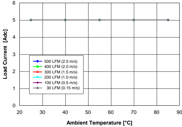
Fig. 1.2V.1: Available load current vs. ambient temperature and airflow rates for V_{out} = 1.2\text{V} converter mounted vertically with V_{in} = 12\text{V} , air flowing from pin 5 to pin 1 and maximum MOSFET temperature \leq 120^{\circ}\text{C} .
