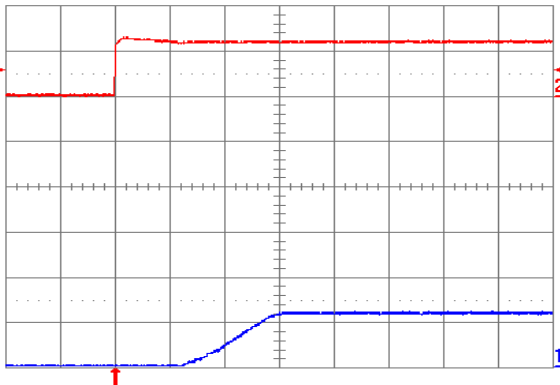
Fig. 1.2V.5: Turn-on transient for V_{out} = 1.2\text{V} with application of V_{in} = 12\text{V} at full rated load current (resistive) and 47\mu\text{F} external capacitance. Top trace: V_{in} (10V/div); Bottom trace: V_{out} (1V/div); Time scale: 2 ms/div.
