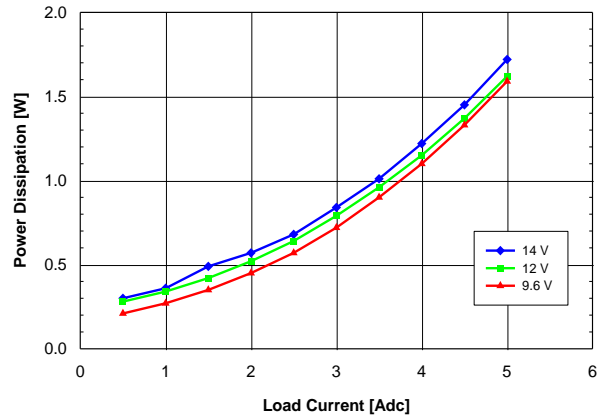
Fig. 1.2V.4: Power Loss vs. load current and input voltage for V_{out} = 1.2\text{V} converter mounted vertically with air flowing from pin 5 to pin 1 at a rate of 200 LFM (1 m/s) and T_a = 25^{\circ}\text{C} .
