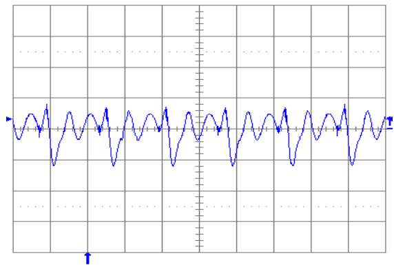
Fig. 1.2V.6: Output voltage ripple (10mv/div) at full rated load current into a resistive load with external capacitance 47\mu\text{F} ceramic + 1\mu\text{F} ceramic and V_{in} = 12\text{V} for V_{out} = 1.2\text{V} . Time scale: 2 \mu\text{s} /div.
