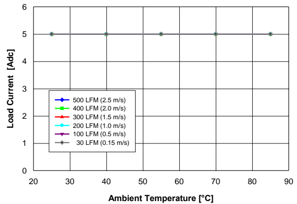
Fig. 1.8V.2: Available load current vs. ambient temperature and airflow rates for V_{out} = 1.8V converter mounted horizontally with V_{in} = 12V , air flowing from pin 5 to pin 1 and maximum MOSFET temperature \leq 120^\circ C .
