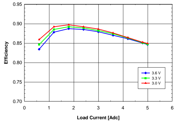
Fig. 1.0V.4: Efficiency vs. load current and input voltage for V_{out} = 1.0\text{ V} converter mounted vertically with air flowing from pin 5 to pin 1 at a rate of 200 LFM (1 m/s) and T_a = 25\text{ }^\circ\text{C} .
