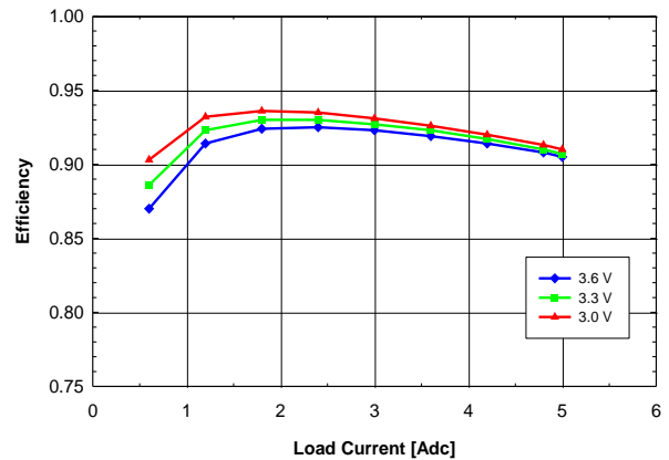
Fig. 1.8V.4: Efficiency vs. load current and input voltage for V_{out} = 1.8\text{ V} converter mounted vertically with air flowing from pin 5 to pin 1 at a rate of 200 LFM (1 m/s) and T_a = 25\text{ }^\circ\text{C} .
