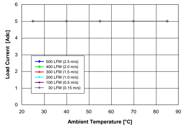
Fig. 1.5V.2: Available load current vs. ambient temperature and airflow rates for V_{out} = 1.5\text{ V} converter mounted horizontally with V_{in} = 5\text{ V} , air flowing from pin 5 to pin 1, and maximum MOSFET temperature \leq 120\text{ }^\circ\text{C} .
