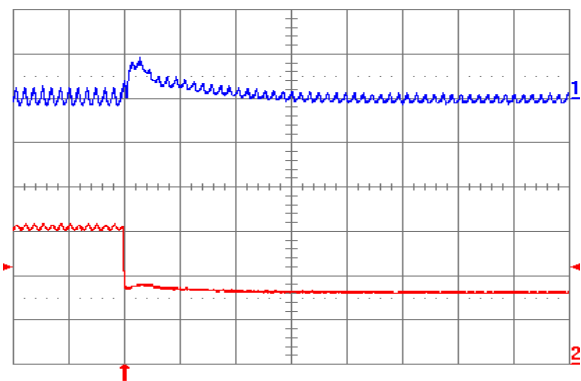
Fig. 0.7525V.8: Output voltage response for V_{out} = 0.7525\text{ V} to negative load current step change from 5 A to 2.5 A with slew rate of -5\text{ A}/\mu\text{s} at V_{in} = 5\text{ V} . Top trace: output voltage (100 mV/div.); Bottom trace: load current (2 A/div.). C_o = 47\text{ }\mu\text{F} ceramic + 1\text{ }\mu\text{F} ceramic. Time scale: 20 \mu\text{s} /div.
