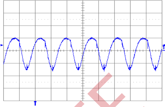
Fig. 3.3V.6: Output voltage ripple (20 mV/div.) at full rated load current into a resistive load with external capacitance 10\ \mu\text{F} ceramic + 1\ \mu\text{F} ceramic and V_{in} = 5\text{ V} for V_{out} = 3.3\text{ V} . Time scale: 2 μs/div.
