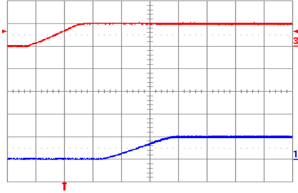
Fig. 1.0V.5: Turn-on transient for V_{out} = 1.0\text{ V} with application of V_{in} at full rated load current (resistive) and 47\ \mu\text{F} external capacitance at V_{in} = 5\text{ V} . Top trace: V_{in} (5 V/div.); Bottom trace: output voltage (1 V/div.); Time scale: 2 ms/div.
