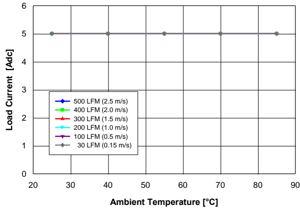
Fig. 1.2V.1: Available load current vs. ambient temperature and airflow rates for V_{out} = 1.2\text{ V} converter mounted vertically with V_{in} = 5\text{ V} , air flowing from pin 5 to pin 1, and maximum MOSFET temperature \leq 120\text{ }^{\circ}\text{C} .
