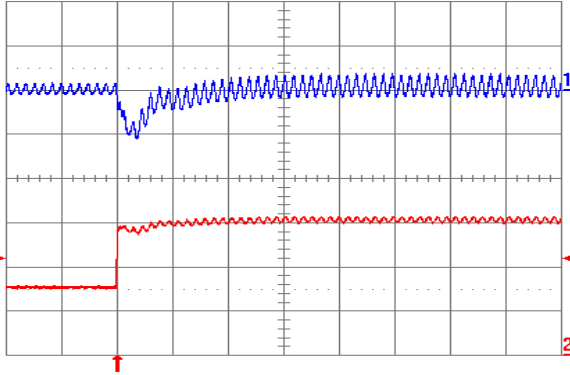
Fig. 1.2V.6: Output voltage response for V_{out} = 1.2\text{ V} to positive load current step change from 2.5 A to 5 A with slew rate of 5\text{ A}/\mu\text{s} at V_{in} = 5\text{ V} . Top trace: output voltage (100 mV/div.); Bottom trace: load current (2 A/div.). C_o = 47\text{ }\mu\text{F} ceramic + 1\text{ }\mu\text{F} ceramic. Time scale: 20\text{ }\mu\text{s}/\text{div} .
