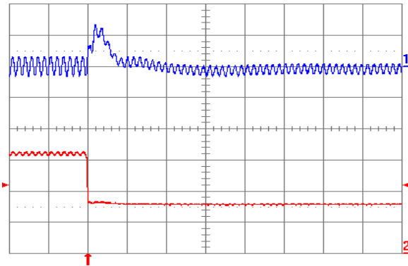
Fig. 2.5V.8: Output voltage response for V_{out} = 2.5\text{ V} to negative load current step change from 5 A to 2.5 A with slew rate of -5\text{ A}/\mu\text{s} at V_{in} = 5\text{ V} . Top trace: output voltage (100 mV/div.); Bottom trace: load current (2 A/div.). C_o = 47\text{ }\mu\text{F} ceramic + 1\text{ }\mu\text{F} ceramic. Time scale: 20 \mu\text{s} /div.
