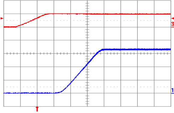
Fig. 3.3V.5: Turn-on transient for V_{out} = 3.3\text{ V} with application of V_{in} at full rated load current (resistive) and 47\ \mu\text{F} external capacitance at V_{in} = 5\text{ V} . Top trace: V_{in} (5 V/div.); Bottom trace: output voltage (1 V/div.); Time scale: 2 ms/div.
