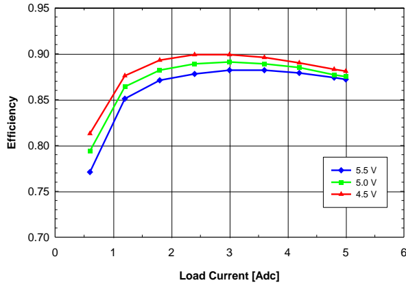
Fig. 1.5V.3: Efficiency vs. load current and input voltage for V_{out} = 1.5\text{ V} converter mounted vertically with air flowing from pin 5 to pin 1 at a rate of 200 LFM (1 m/s) and T_a = 25\text{ }^\circ\text{C} .
