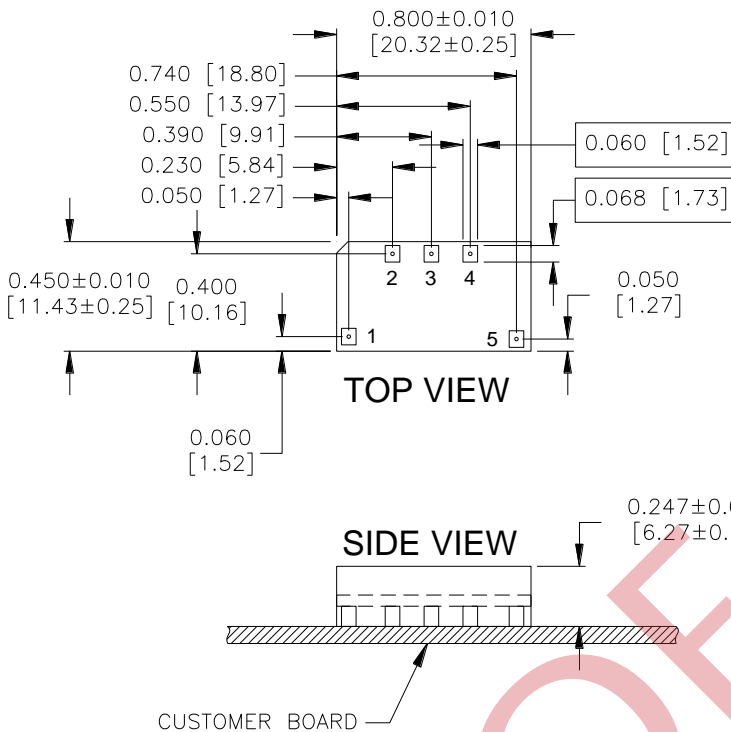
YNM05S Pinout (Surface Mount)
