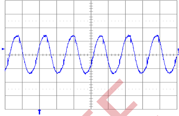
Fig. 1.8V.6: Output voltage ripple ( 20\text{ mV/div.} ) at full rated load current into a resistive load with external capacitance 10\text{ }\mu\text{F} ceramic + 1\text{ }\mu\text{F} ceramic and V_{in} = 5\text{ V} for V_{out} = 1.8\text{ V} . Time scale: 2\text{ }\mu\text{s/div.}
