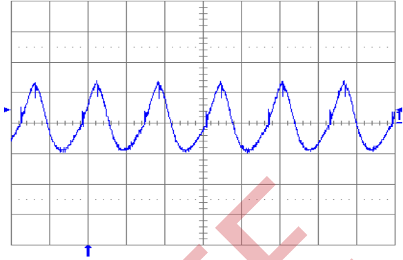
Fig. 1.0V.6: Output voltage ripple (20 mV/div.) at full rated load current into a resistive load with external capacitance 10\ \mu\text{F} ceramic + 1\ \mu\text{F} ceramic and V_{in} = 5\text{ V} for V_{out} = 1.0\text{ V} . Time scale: 2 \mu\text{s} /div.
