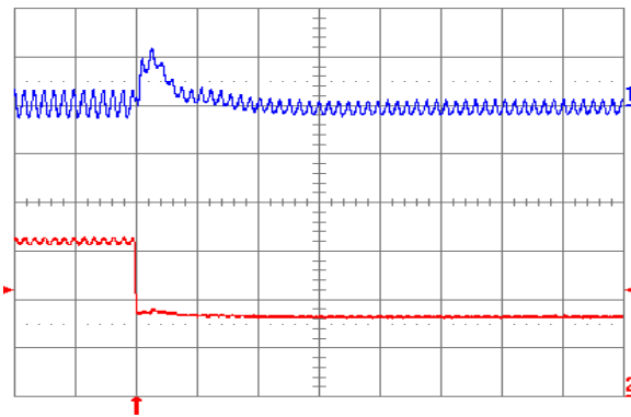
Fig. 1.5V.8: Output voltage response for V_{out} = 1.5\text{ V} to negative load current step change from 5 A to 2.5 A with slew rate of -5 A/ \mu\text{s} at V_{in} = 5\text{ V} . Top trace: output voltage (100 mV/div.); Bottom trace: load current (2 A/div.). C_o = 47\text{ }\mu\text{F} ceramic + 1 \mu\text{F} ceramic. Time scale: 20 \mu\text{s} /div.
