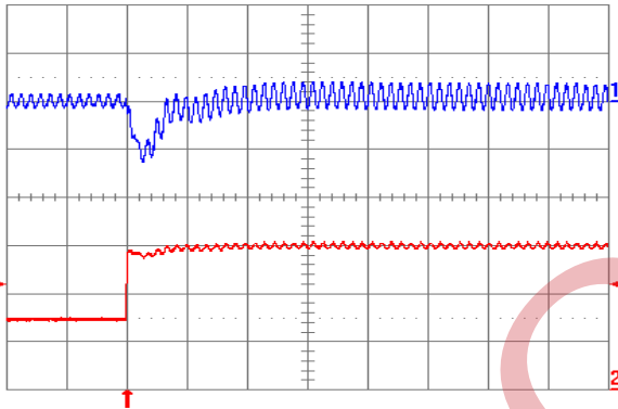
Fig. 1.8V.7: Output voltage response for V_{out} = 1.8\text{ V} to positive load current step change from 2.5\text{ A} to 5\text{ A} with slew rate of 5\text{ A}/\mu\text{s} at V_{in} = 5\text{ V} . Top trace: output voltage ( 100\text{ mV/div.} ); Bottom trace: load current ( 2\text{ A/div.} ). C_o = 47\text{ }\mu\text{F} ceramic + 1\text{ }\mu\text{F} ceramic. Time scale: 20\text{ }\mu\text{s/div.}
