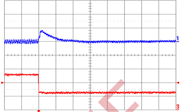
Fig. 5.0V.8: Output voltage response for V_{out} = 5.0\text{ V} to negative load current step change from 5\text{ A} to 2.5\text{ A} with slew rate of -5\text{ A}/\mu\text{s} at V_{in} = 12\text{ V} . Top trace: output voltage ( 100\text{ mV}/\text{div.} ); Bottom trace: load current ( 2\text{ A}/\text{div.} ). C_o = 47\text{ }\mu\text{F} ceramic. Time scale: 20\text{ }\mu\text{s}/\text{div.}
