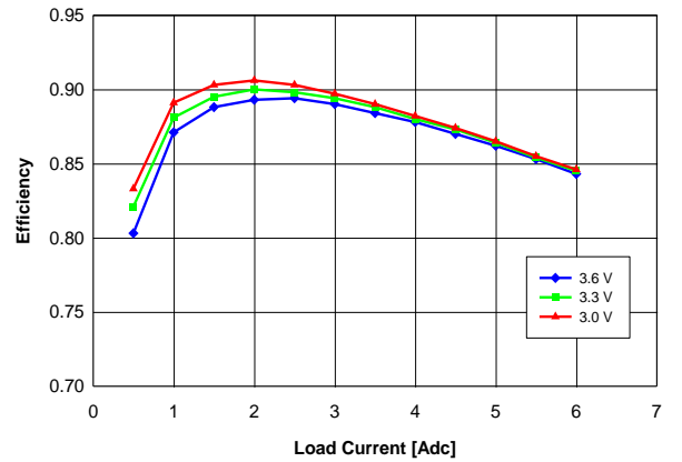
Fig. 1.2V.4: Efficiency vs. load current and input voltage for V_{out} = 1.2V converter mounted vertically or horizontally with air flowing from pin 5 to pin 1 at a rate of 200 LFM (1 m/s) and T_a = 25^{\circ}C .
