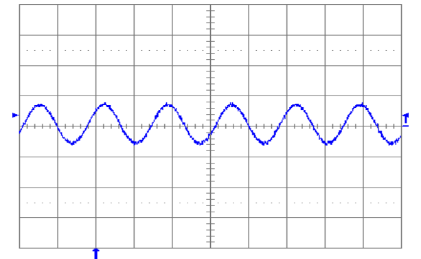
Fig. 1.2V.6: Output voltage ripple (20mV/div.) at full rated load current into a resistive load with external capacitance 47\mu F ceramic + 1\mu F ceramic and V_{in} = 5V for V_{out} = 1.2V . Time scale: 2µs/div.
