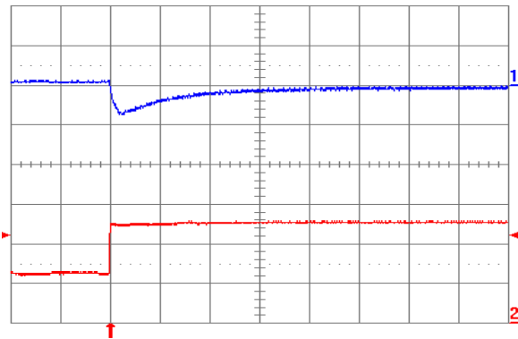
Fig. 1.0V.7: Output voltage response for V_{out} = 1.0\text{ V} to positive load current step change from 2.5\text{ A} to 5\text{ A} with slew rate of 5\text{ A}/\mu\text{s} at V_{in} = 12\text{ V} . Top trace: output voltage ( 100\text{ mV/div.} ); Bottom trace: load current ( 2\text{ A/div.} ). C_o = 100\ \mu\text{F} ceramic. Time scale: 20\ \mu\text{s/div.}
