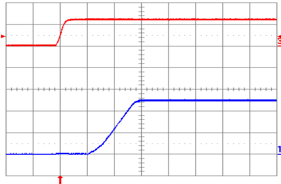
Fig. 2.5V.5: Turn-on transient for V_{out} = 2.5\text{ V} with application of V_{in} at full rated load current (resistive) and 100 \mu\text{F} external capacitance at V_{in} = 12\text{ V} . Top trace: V_{in} (10 V/div.); Bottom trace: output voltage (1 V/div.); Time scale: 5 ms/div.
