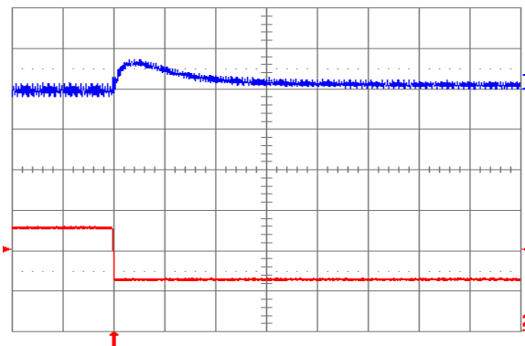
Fig. 1.2V.8: Output voltage response for V_{out} = 1.2\text{ V} to negative load current step change from 5 A to 2.5 A with slew rate of -5\text{ A}/\mu\text{s} at V_{in} = 12\text{ V} . Top trace: output voltage (100 mV/div.); Bottom trace: load current (2 A/div.). C_o = 100\text{ }\mu\text{F} ceramic. Time scale: 20\text{ }\mu\text{s}/\text{div} .
