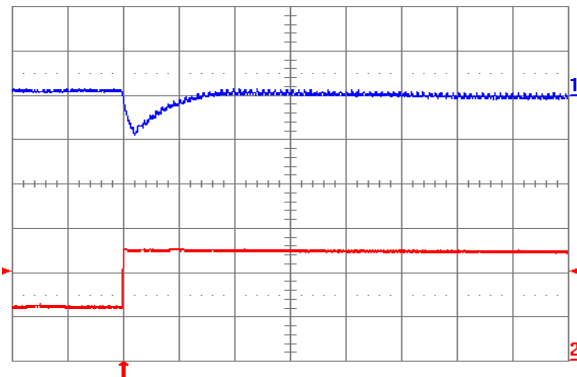
Fig. 2.5V.7: Output voltage response for V_{out} = 2.5\text{ V} to positive load current step change from 2.5 A to 5 A with slew rate of 5 A/ \mu\text{s} at V_{in} = 12\text{ V} . Top trace: output voltage (100 mV/div.); Bottom trace: load current (2 A/div.). C_o = 100\text{ } \mu\text{F} ceramic. Time scale: 20 \mu\text{s} /div.
