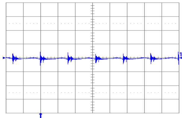
Fig. 1.2V.6: Output voltage ripple (20mV/div.) at full rated load current into a resistive load with external capacitance 100\mu F ceramic and V_{in} = 12V for V_{out} = 1.2V . Time scale: 2μs/div.
