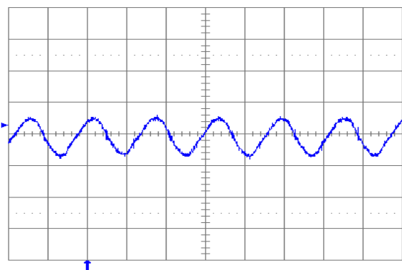
Fig. 5.0V.6: Output voltage ripple (20mV/div.) at full rated load current into a resistive load with external capacitance 100\mu F ceramic and V_{in} = 12V for V_{out} = 5.0V . Time scale: 2\mu s /div.
