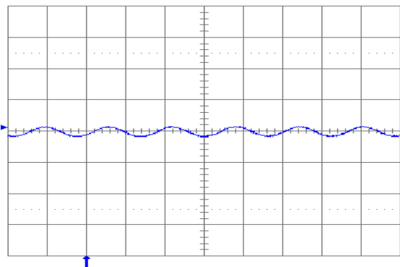
Fig. 1.8V.6: Output voltage ripple (20mV/div.) at full rated load current into a resistive load with external capacitance 100\mu F ceramic and V_{in} = 12V for V_{out} = 1.8V . Time scale: 2\mu s /div.
