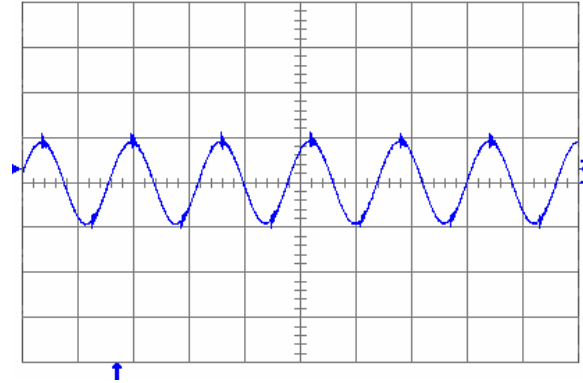
Fig. 2.5V.6: Output voltage ripple (20 mV/div.) at full rated load current into a resistive load with external capacitance 100\ \mu\text{F} ceramic + 1\ \mu\text{F} ceramic and V_{in} = 5\text{ V} for V_{out} = 2.5\text{ V} . Time scale: 2 \mu\text{s} /div.
