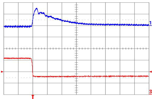
Fig. 3.3V.8: Output voltage response for V_{out} = 3.3\text{ V} to negative load current step change from 16 A to 8 A with slew rate of -5\text{ A}/\mu\text{s} at V_{in} = 5\text{ V} . Top trace: output voltage (100 mV/div.); Bottom trace: load current (5 A/div.). C_o = 100\text{ }\mu\text{F} ceramic. Time scale: 20 \mu\text{s} /div.
