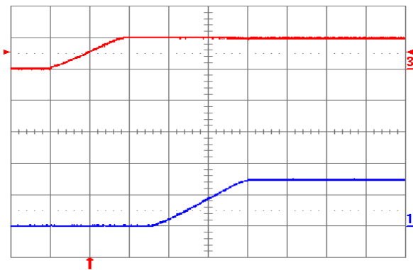
Fig. 1.5V.5: Turn-on transient for V_{out} = 1.5 V with application of V_{in} at full rated load current (resistive) and 100 \mu F external capacitance at V_{in} = 5 V. Top trace: V_{in} (5 V/div.); Bottom trace: output voltage (1 V/div.); Time scale: 2 ms/div.
