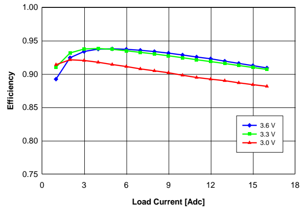
Fig. 2.5V.4: Efficiency vs. load current and input voltage for V_{out} = 2.5\text{ V} converter mounted vertically with air flowing at a rate of 200 LFM (1 m/s) and T_a = 25^\circ\text{C} .
