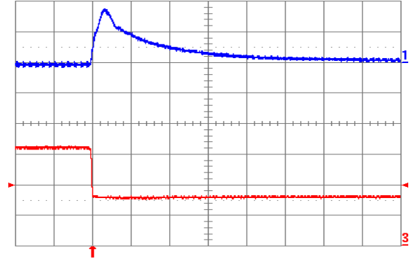
Fig. 0.7525V.8: Output voltage response for V_{out} = 0.7525 V to negative load current step change from 16 A to 8 A with slew rate of -5 A/ \mu s at V_{in} = 5 V. Top trace: output voltage (100 mV/div.); Bottom trace: load current (5 A/div.). C_o = 100 \mu F ceramic. Time scale: 20 \mu s/div.
