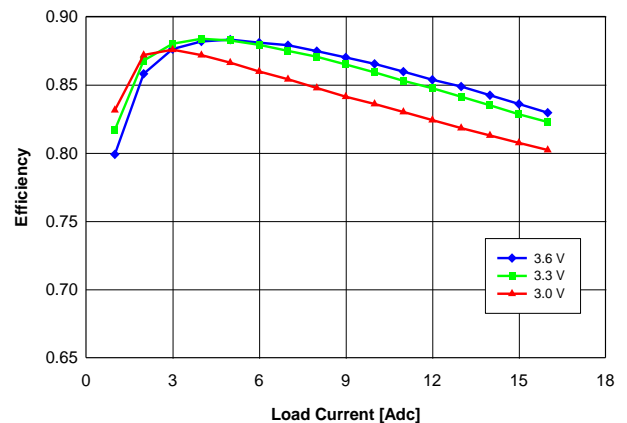
Fig. 1.2V.4: Efficiency vs. load current and input voltage for V_{out} = 1.2\text{ V} converter mounted vertically with air flowing at a rate of 200 LFM ( 1\text{ m/s} ) and T_a = 25\text{ }^\circ\text{C} .
