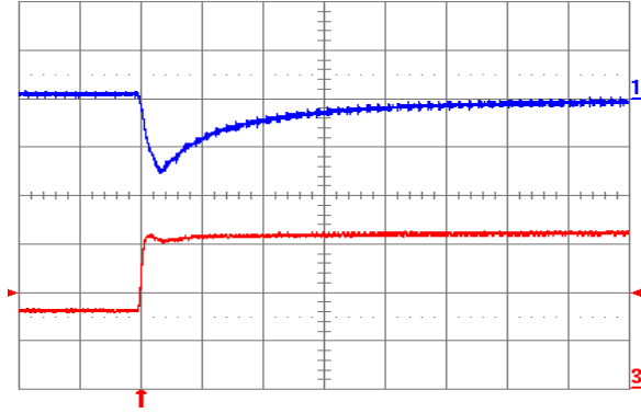
Fig. 0.7525V.7: Output voltage response for V_{out} = 0.7525 V to positive load current step change from 8 A to 16 A with slew rate of 5 A/ \mu s at V_{in} = 5 V. Top trace: output voltage (100 mV/div.); Bottom trace: load current (5 A/div.). C_o = 100 \mu F ceramic. Time scale: 20 \mu s/div.
