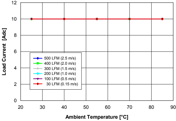
Fig. 1.2V.1: Available load current vs. ambient temperature and airflow rates for V out = 1.2 V converter mounted vertically with V in = 12 V, and maximum MOSFET temperature ≤ 110 °C.
