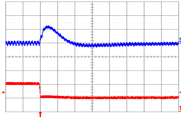
Fig. 1.8V.8: Output voltage response for V_{out} = 1.8 V to negative load current step change from 10 A to 5 A with slew rate of -5 \text{ A}/\mu\text{s} at V_{in} = 12 V. Top trace: output voltage (100 mV/div.); Bottom trace: load current (5 A/div.). C_o = 100 \mu\text{F} ceramic. Time scale: 20 \mu\text{s}/\text{div} .
