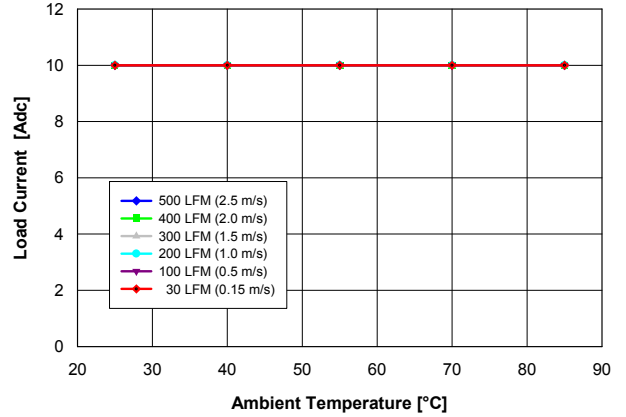
Fig. 1.2V.2: Available load current vs. ambient temperature and airflow rates for V out = 1.2 V converter mounted horizontally with V in = 12 V, and maximum MOSFET temperature ≤ 110 °C.
