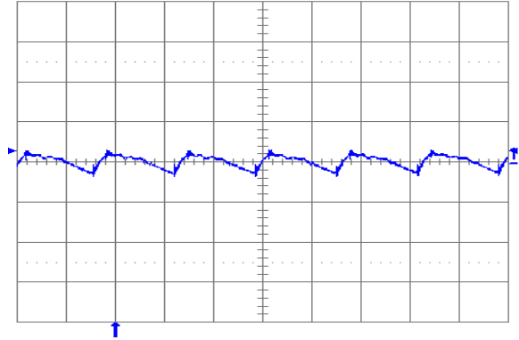
Fig. 1.8V.6: Output voltage ripple (20 mV/div.) at full rated load current into a resistive load with external capacitance 100 \mu\text{F} ceramic + 1 \mu\text{F} ceramic, and V_{in} = 12 V for V_{out} = 1.8 V. Time scale: 2 \mu\text{s}/\text{div} .
