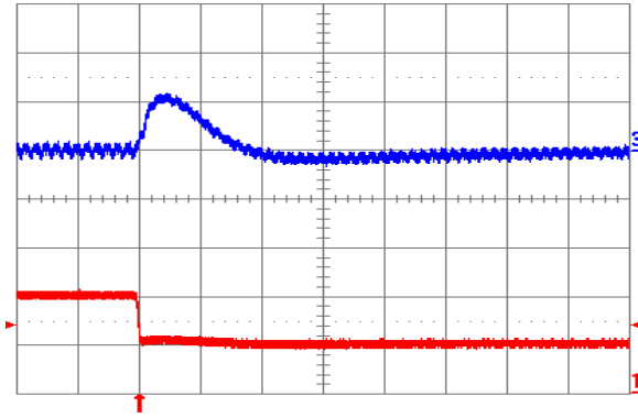
Fig. 1.5V.8: Output voltage response for V_{out} = 1.5 V to negative load current step change from 10 A to 5 A with slew rate of -5 \text{ A}/\mu\text{s} at V_{in} = 12 V. Top trace: output voltage (100 mV/div.); Bottom trace: load current (2 A/div.). C_o = 100 \mu\text{F} ceramic. Time scale: 20 \mu\text{s} /div.
