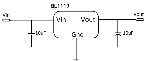
Application circuit of BL1117 fixed version
