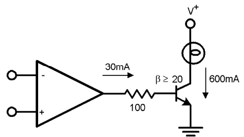
Lamp Driver
