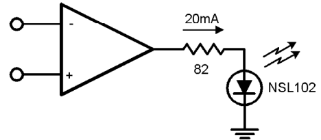
LED Driver
