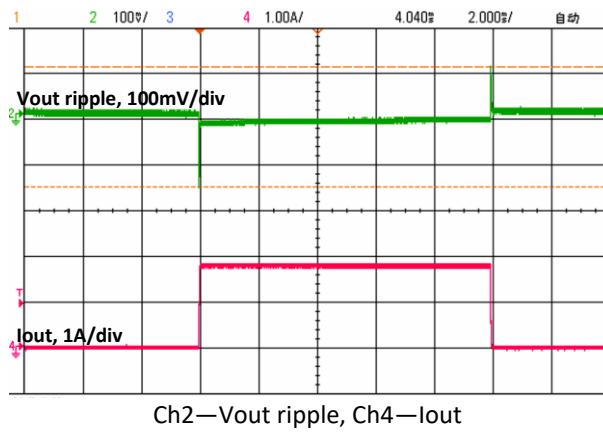
V_{in}=5V / V_{out}=1.8V / I_{out}=0.01\sim 1.8A
