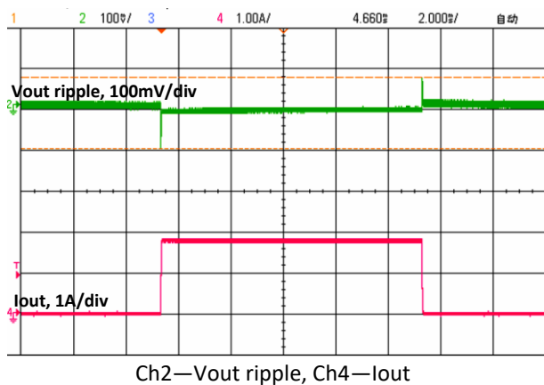
V_{in}=5V / V_{out}=1.2V / I_{out}=0.01\sim 1.8A
