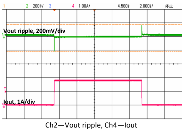
V_{in}=5V / V_{out}=2.5V / I_{out}=0.01\sim 1.8A
