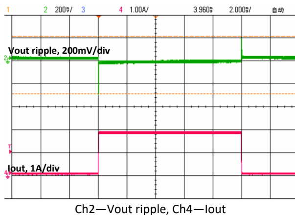
V_{in}=5V / V_{out}=3.3V / I_{out}=0.01\sim 1.8A
