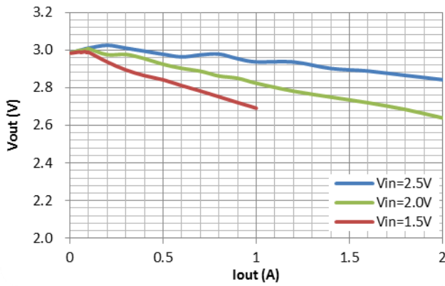
BL8531C CB5TR30 Output Voltage VS Output Current
