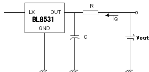
Quiescent current test circuit ( V_{out}=V_{out\_nom} \times 1.05 , R=1K\Omega , C=0.1\mu F )
