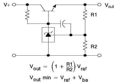
Series Pass Regulator
