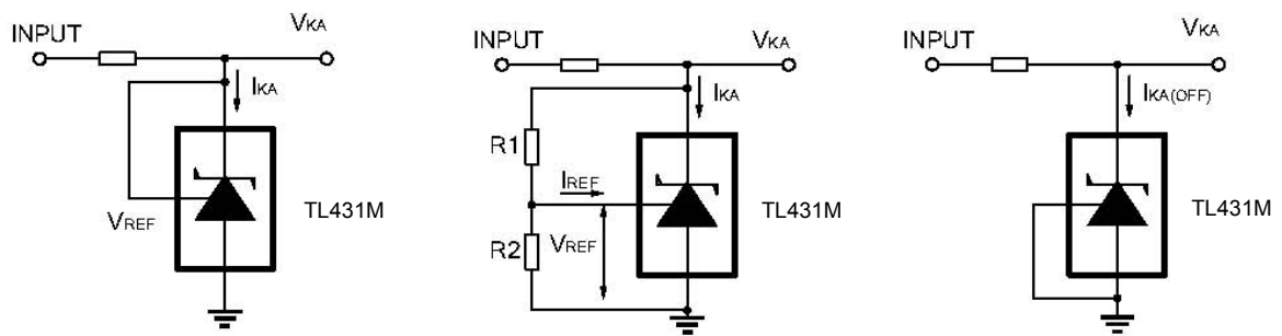
Test Circuit For V_{KA}=V_{REF}
