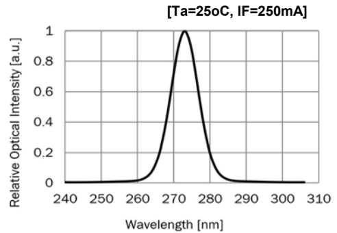
FIG 4. Spectrum
