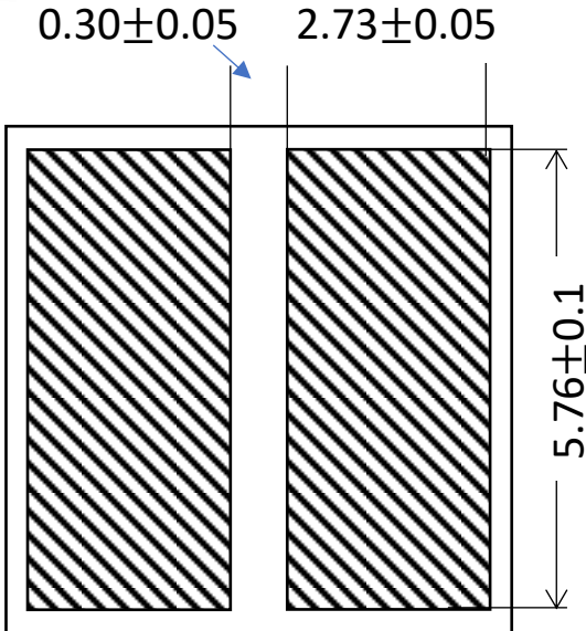
Recommended Solder Pattern on PCB
