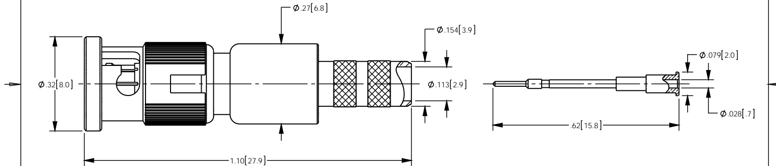
RECOMMENDED CABLE STRIPPING DIM'S
