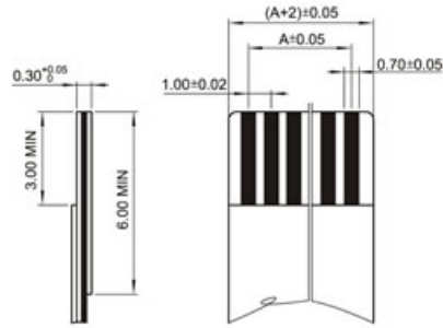
Proper Cable
