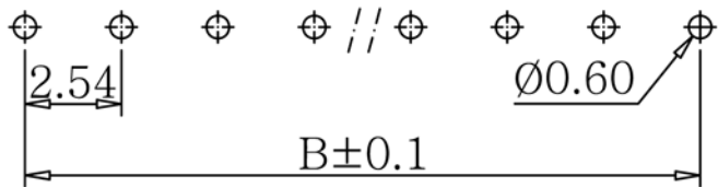
P. C. B Layout
