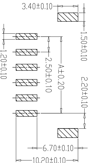
PCB LAYOUT
