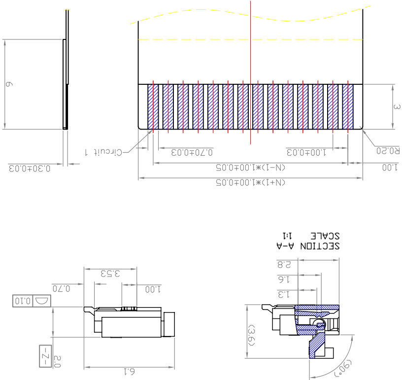
RECOMMENDED FPC/FPC DIMENSION
