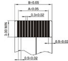
Proper Cable
