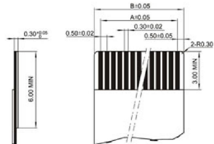
Proper Cable
