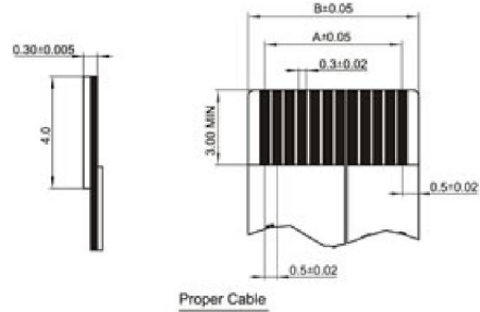
Proper Cable
