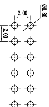
PCB LAYOUT
