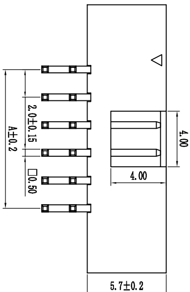
PCB LAYOUT
