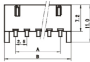
安装尺寸 MOUNTING MEASUREMENT
